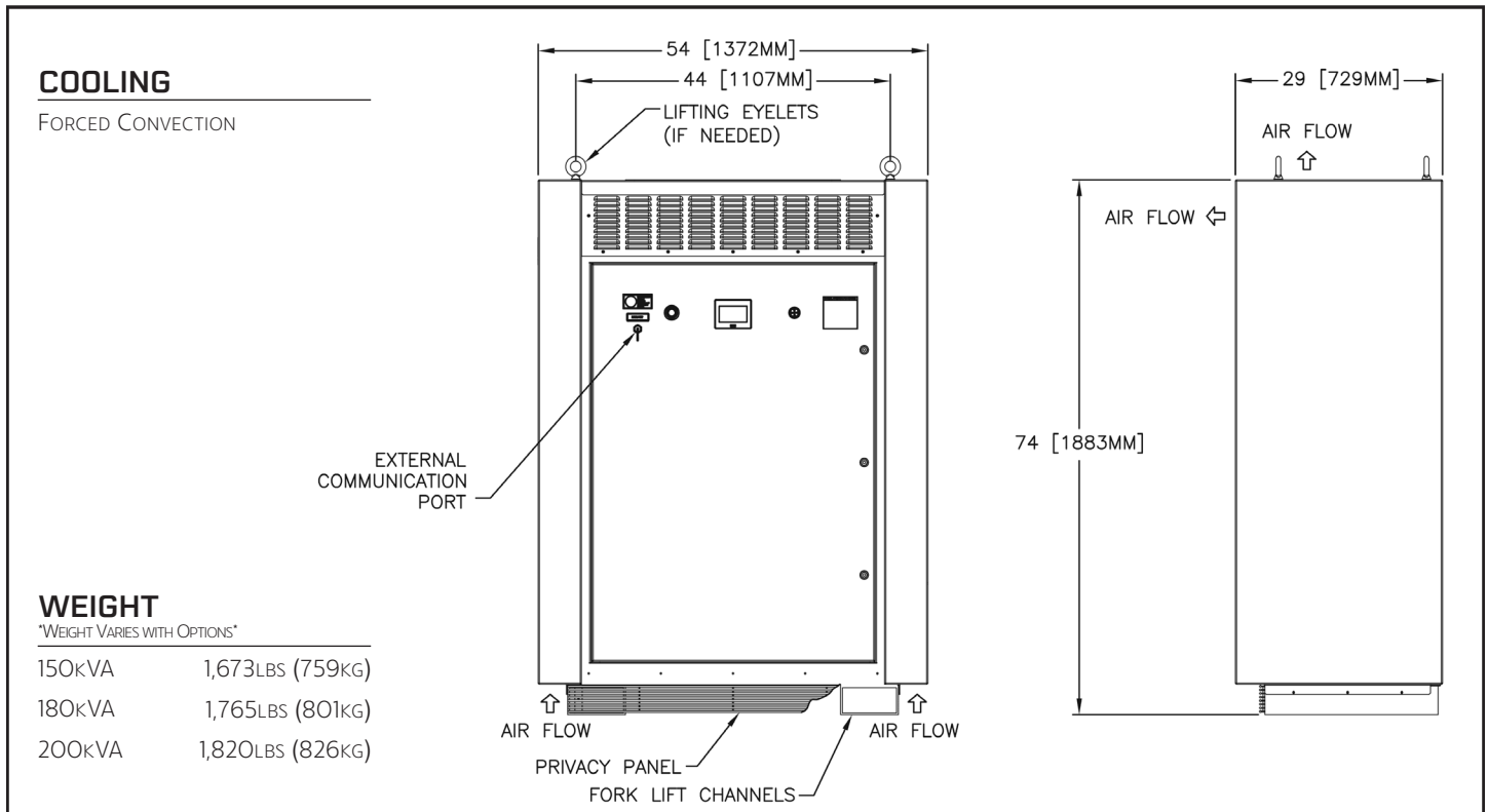
FIGURE 1 – ShoPOWER Ultra HF 150–200kVA
